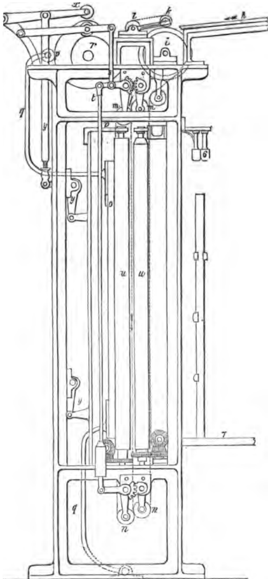
Plate 4.—END VIEW OF FEEDING APPARATUS.
